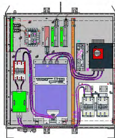
DCIT Gun Station Control with Ground Safety Monitoring & 10 - 30mA Personnel Protection System
